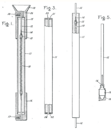
1918 Brevet Charles Abbott
